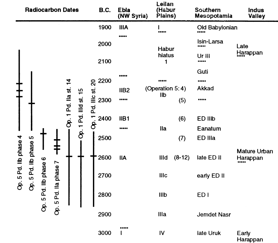
Fig. 4. Third millennium B.C. Southwest Asia chronology. Vertical lines are calibrated ranges \pm 1 SD in years B.C. of Tell Leilan radiocarbon dates for periods IIId through IIb; horizontal lines are calibrated weighted averages. Ebla occupation periods define proto- and early historic chronology for northwest Syria. Leilan ceramically defined periods are subdivided for operation 5 occupation phases. Dates for third millennium historical periods in southern Mesopotamia have an uncertainty of 120 years (67); ED, Early Dynastic. Indus Valley periods are radiocarbon-based estimates (74).
