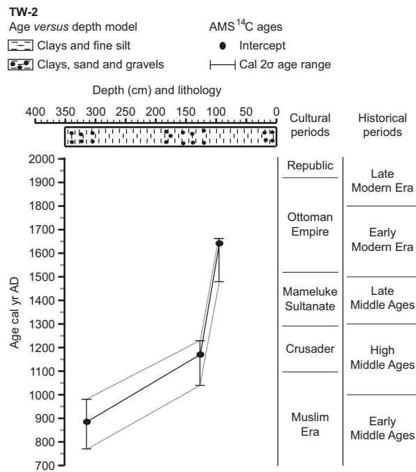
Figure 2. AMS 14 C calibrated ages and suggested age–depth curves
